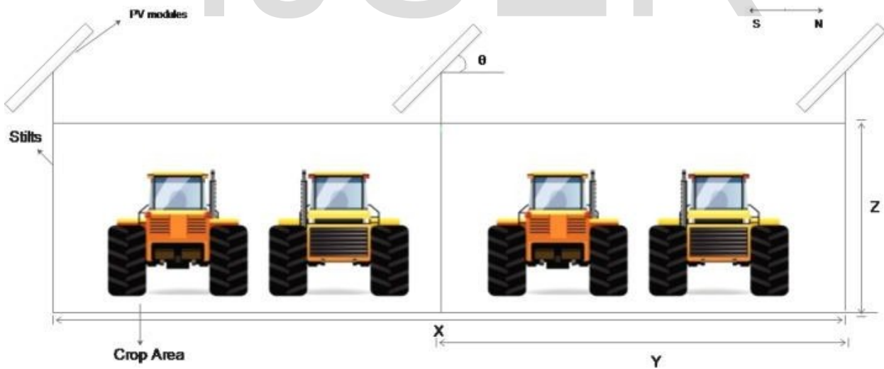
Fig. 1. Agrivoltaic farm schematic having ground mounted PV modules with the area between the panels being used for farming. The spacing between the PV modules has been kept wide enough to allow standard sized farming equipment to pass between the rows.
